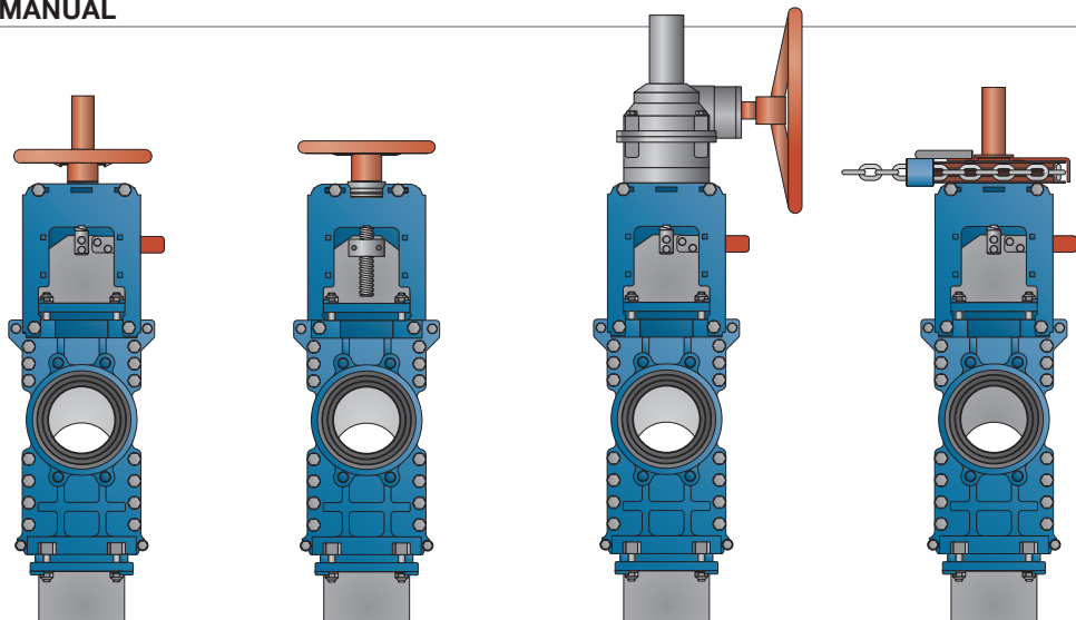
HP-VA Handwheel with rising stem
