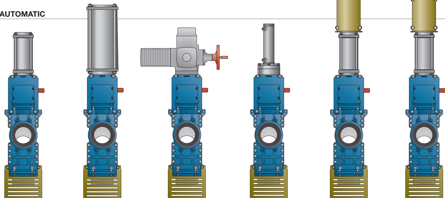
HP-NDE Pneumatic cylinder
